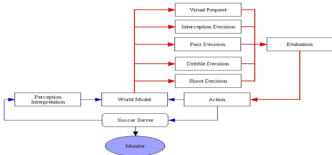
Figure 3. Agent Architecture
