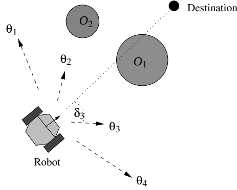
Fig. 1. Evaluation of directions to avoid obstacles.
