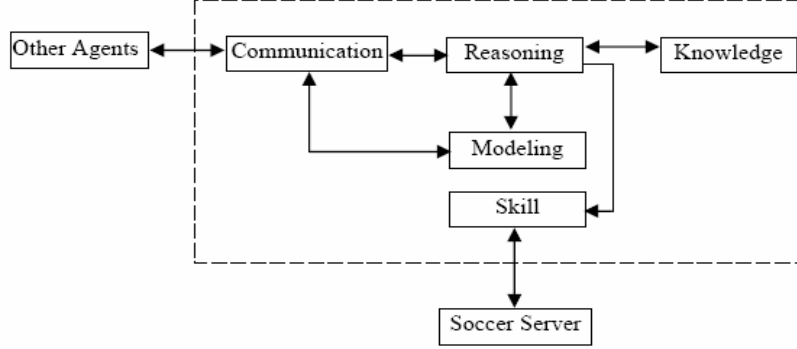
Fig.1. SEU-2D Agent Architecture
