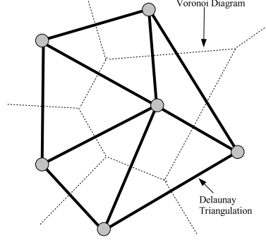
Fig. 2. Example of Delaunay Triangulation
