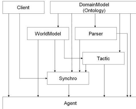
Fig. 1. Dependencies between the modules of the daianmite agent architecture
