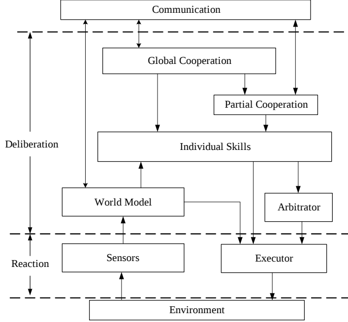
Fig. 1. Decision Architecture of OxBlue2008
