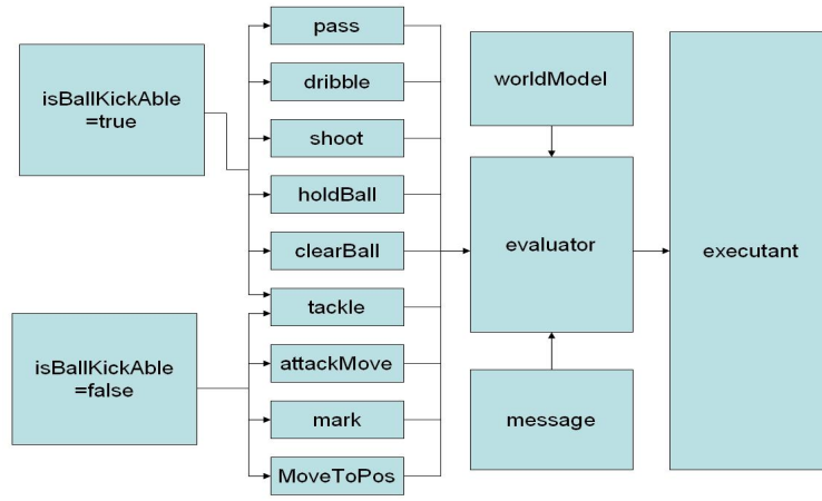
Fig. 1. The structure of HfutEngine2D.
