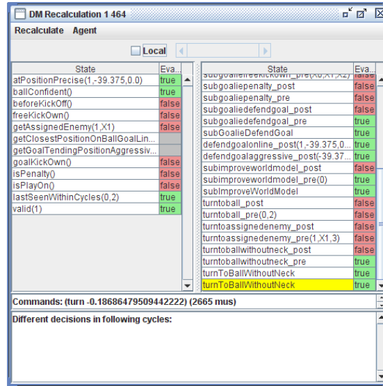
Fig. 7. Decision-Making Recalculation
