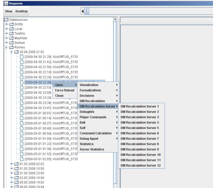
Fig. 8. Datasource View
