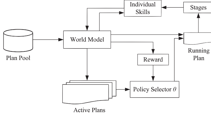
Fig. 5. Learning Process in PSP algorithm
