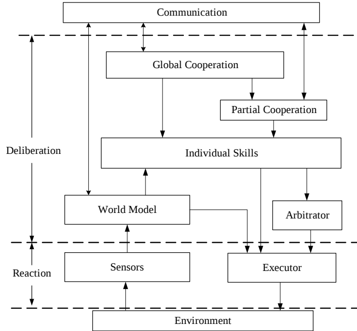
Fig. 1. Decision Architecture of OxBue2009
