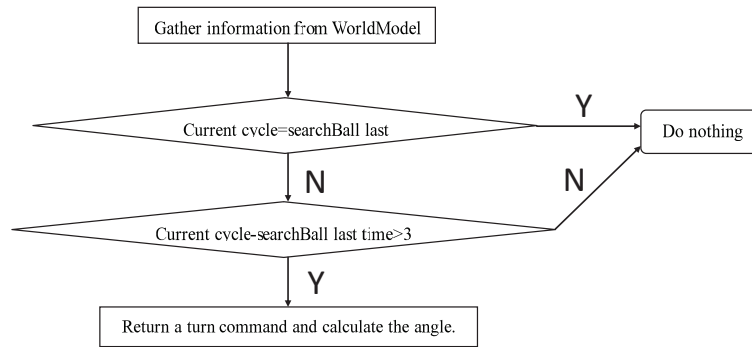
Fig. 3. Diagram of SearchBall
