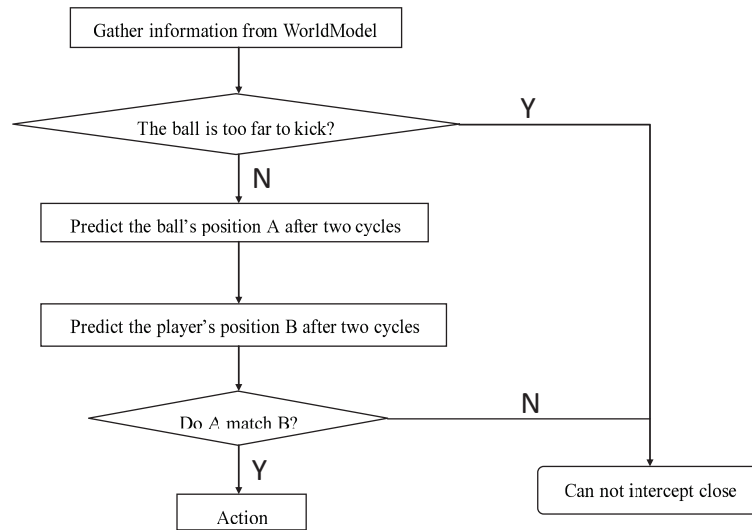
Fig. 4. The Diagram of Intercept Close
