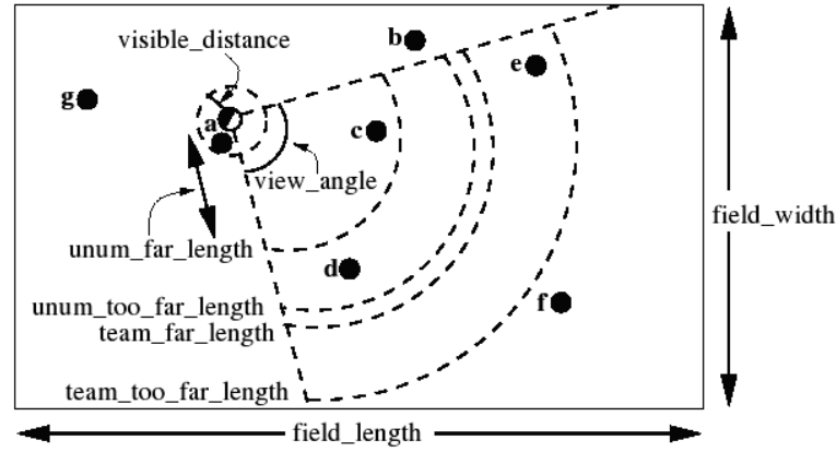
Fig. 2. The Player's Visual Range
