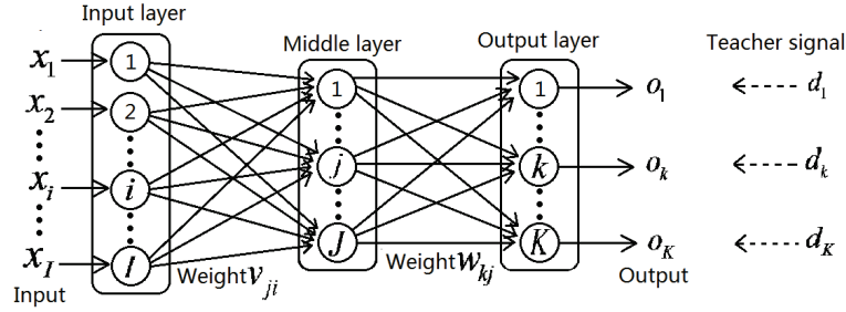
Fig. 1. The Structure of Hierarchical Neural Network
