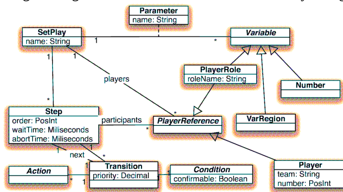
Figure 1. Setplays definition general structure
