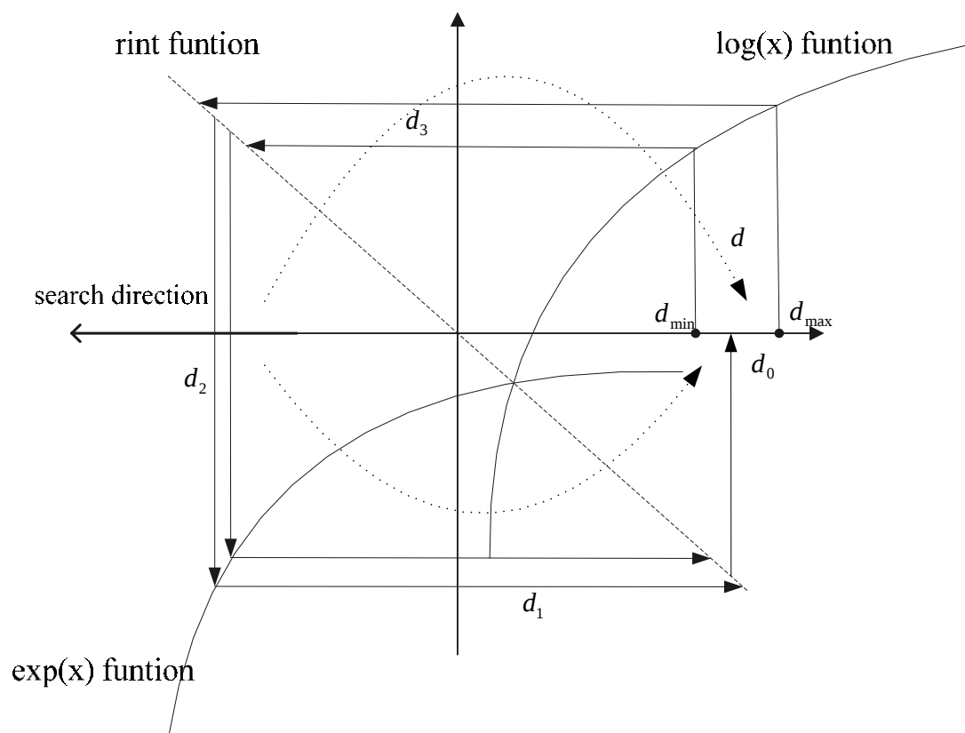
Fig2.2.1 the mapping with logarithmic function, index function and integer function
