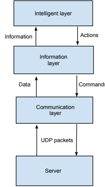
Fig. 1. Software architecture
