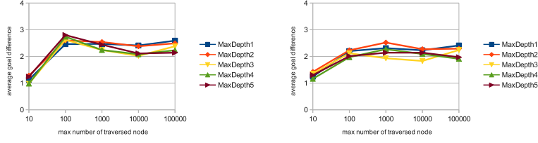
(a) ActionGenerator: Normal type. (b) ActionGenerator: Reduced type. FieldEvaluator: Complex type. FieldEvaluator: Complex type.
