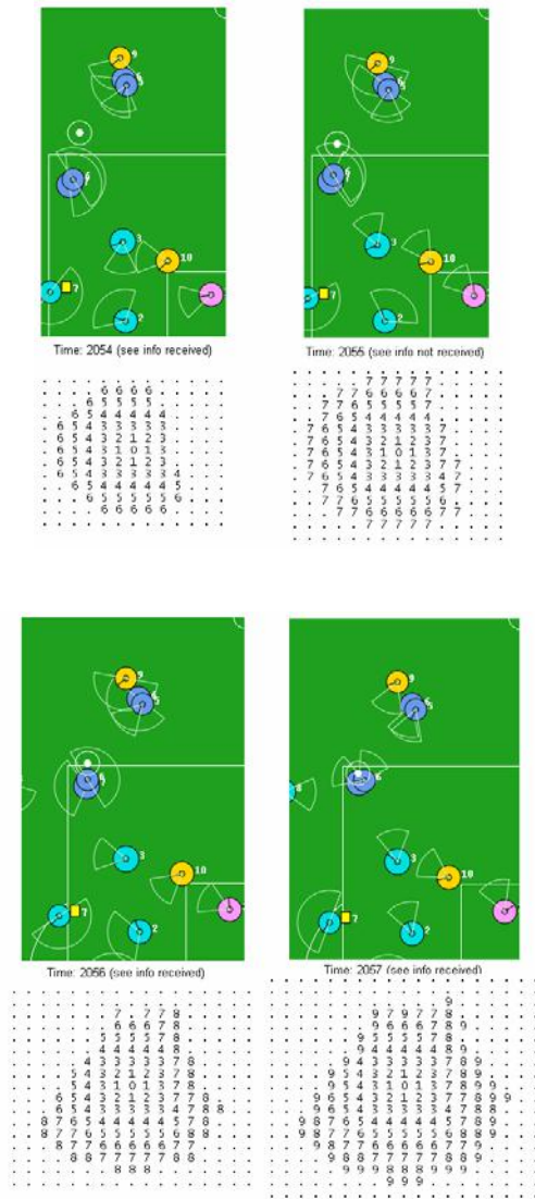
Fig. 2. Our teammate with number 7, adjusts map’s positions of opponent with number 7, using “see” information received.
