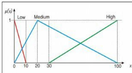
Fig. 3 – % Successful Defenses [6].
