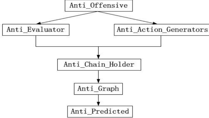
Figure 1: Structure of Anti-Calculation
