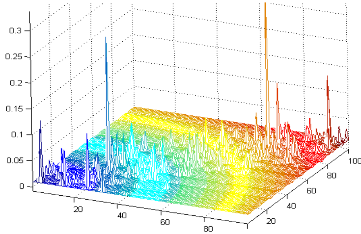
Fig. 3. Transfer matrix of Markov source
