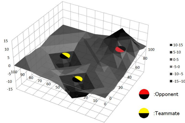
Fig. 1. Image chart of Gravity Field Method
