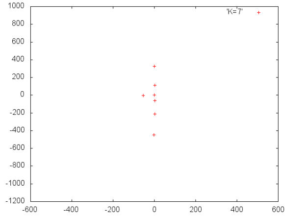
Fig. 3. The average of centers calculated on 10 times of K-means clustering
