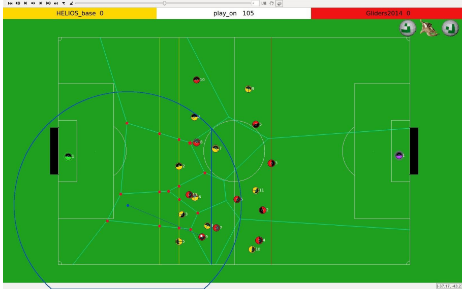
Fig. 1. The mechanism implementing S = \text{tactics}(a) . Voronoi diagram in the game between agent2d (left team) and Gliders2014 (right team) is shown at time = 105, with the n points given by n = 11 agent2d players (yellow/green circles). Light-blue lines show Voronoi segments. The dark-blue line, originating from Gliders player 9, indicates a possible action, a , terminating at possible resultant state S(a) , marked by a blue dot. A subset of possible attacking nodes V'(a) is shown with red dots, within the constraints shown by the dark-blue circle around state S(a) , and the dark-blue line set behind the x -coordinate of S(a) . The best attacking node is marked with a small red star.
