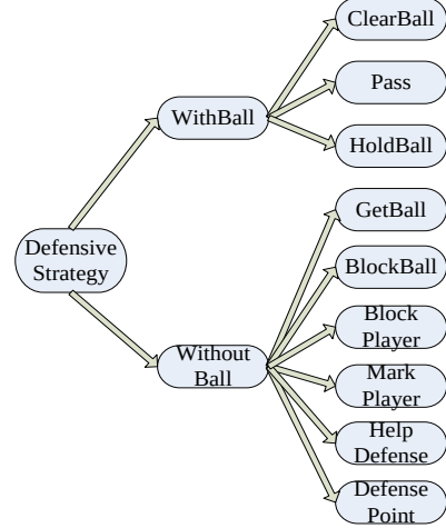
Fig 2 YuShan2015 Defensive Framework
