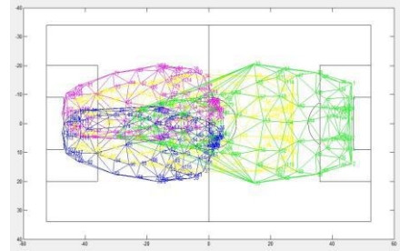
Fig 4 Agent2D 2,3,6,11 formation
