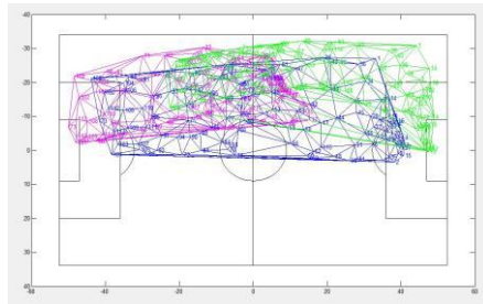
Fig 3 Agent2D 4,7,9 formation
