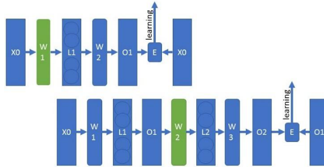
Fig. 1: Comparison between Normal Neural Network and Auto-Encoder
