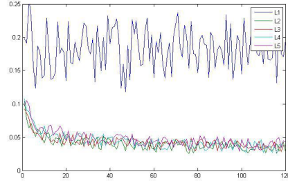
(a) Learn W_1 MLP & Auto-Encoder
