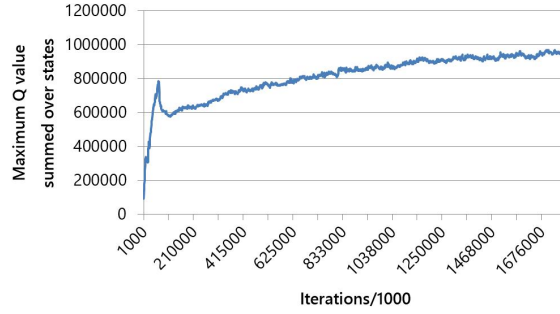
Fig. 6. Maximum Q value summed over states at each 1000 iterations
