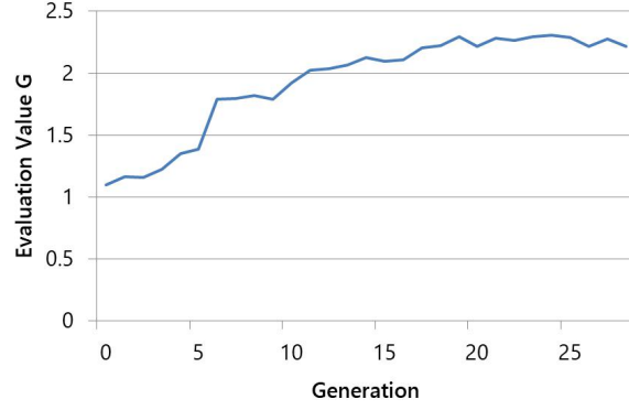
Fig. 5. The best evaluation value G at each generation
