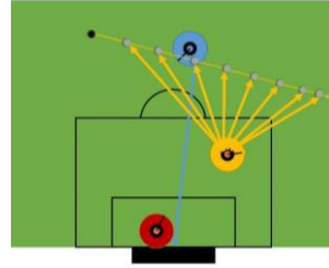
Fig. 2. Intercept Algorithm
