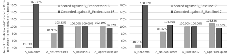
Fig. 2. Taking FRA-UNITed version A_Baseline17 as the ground truth, these charts visualize the relative changes in the average numbers of goals scored and goals conceded when the other three considered versions are matched against Team B (left: against Helios 2016, right: against Helios 2017).
