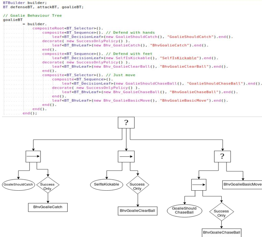
Fig. 3. Code for building our goalie behavior tree and the tree built.
