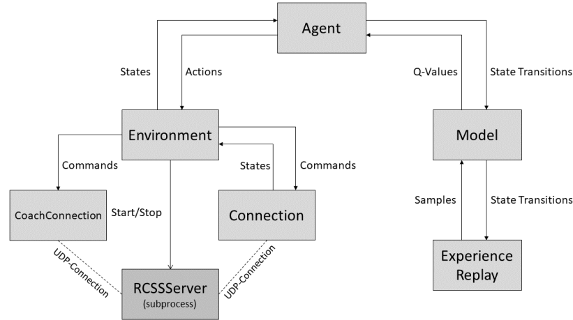
Fig. 2. Overview of the agent’s classes and their relationship in the context of the learning process. Source: [7]
