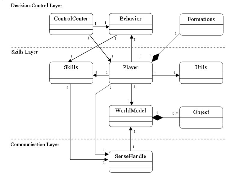
Fig. 1. DeltaAgent Architecture
