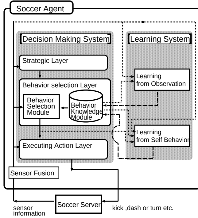
Fig.1. The agent architecture
