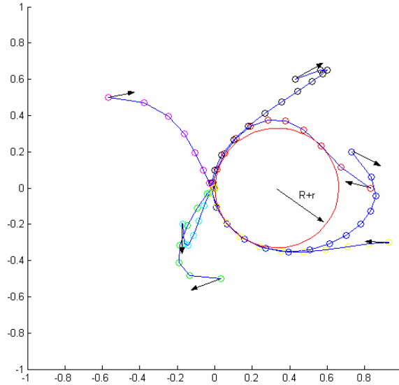
Figure 2 Some cases in path planning. In these cases agent is located in various positions with different velocity and the target is to run to a specific position relative to the ball without colliding with it. Here we assume that the ball is not moving. If the distance of positions in the path and ball is larger than the sum of the radius of ball r and the agent R this requirement is satisfied.
