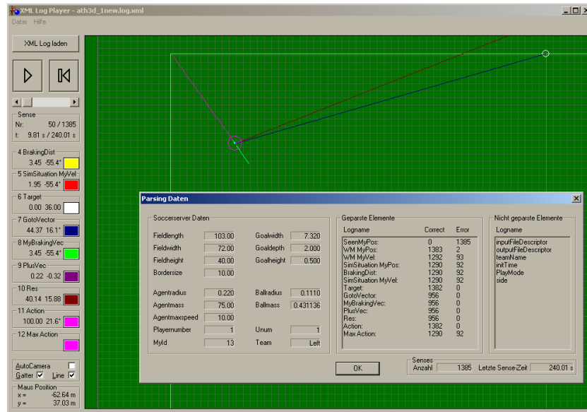
Fig. 2. Present logplayer for play back and graphical analysis of xml logfiles generated by ATH-3D.
