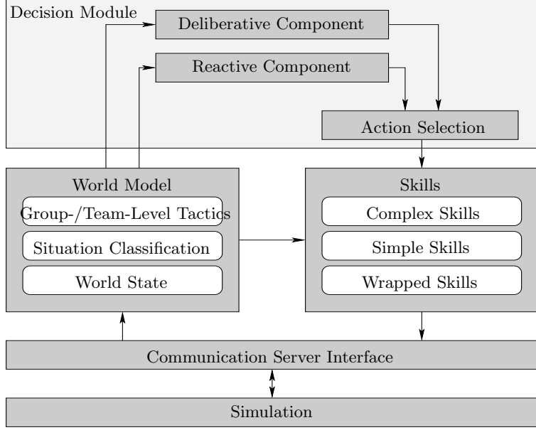
Fig. 1: DR-Architecture adapted to RoboCup 3D soccer simulation
