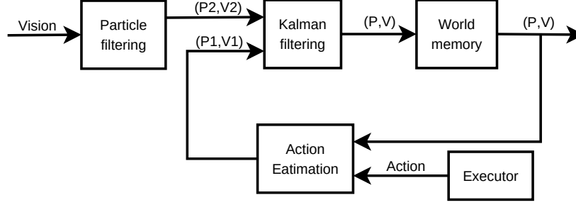
Fig. 2. SEU-3D Self-localization filtering.
