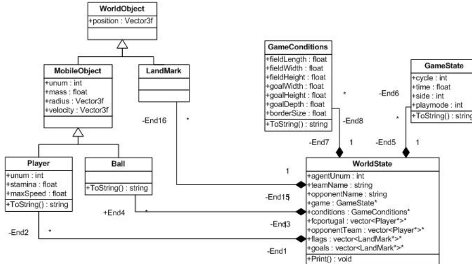
Figure 2: WorldState architecture
