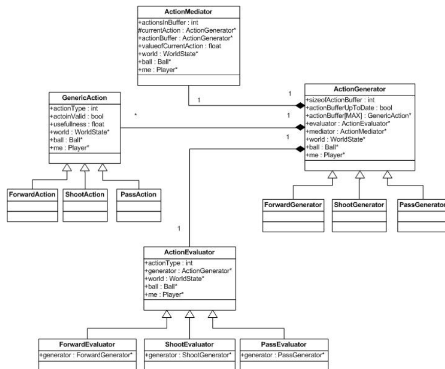
Figure 3 – Actions Architecture.
