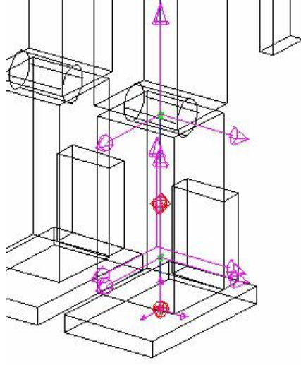
Fig. 3. A frame in the foot for computing the center of pressure relative to the robot's torso.
