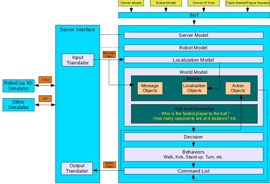
Fig. 2. Borregos3D architecture.
