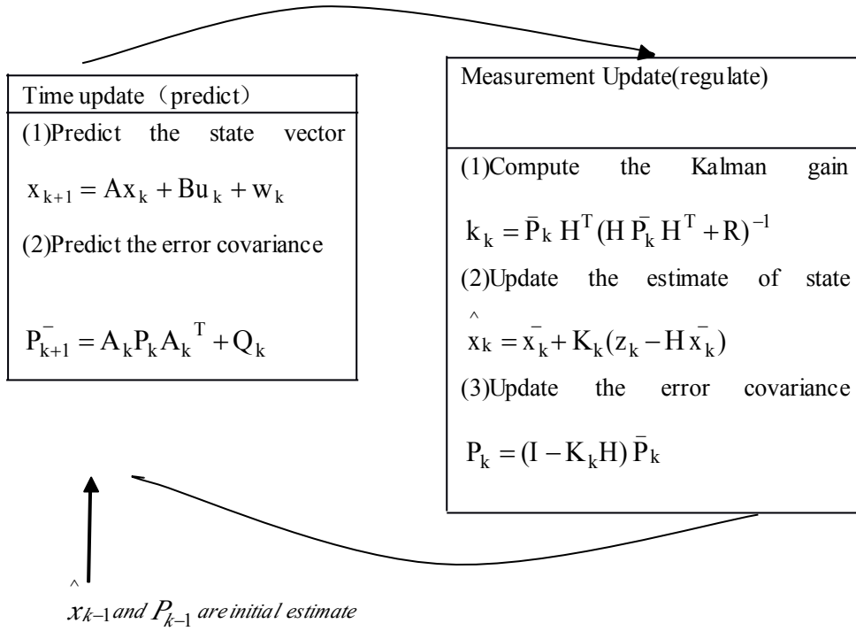
Fig. 1 Kalman filter
