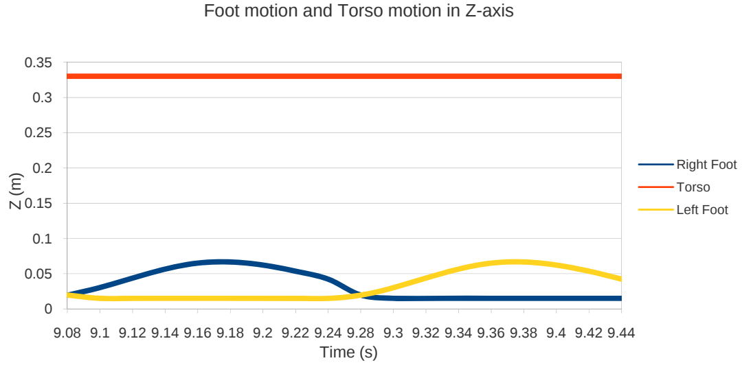
Fig5. Foot motion and torso motion in Z-axis
