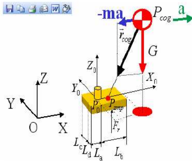
Fig.4. 3-D Inverted Pendulum
