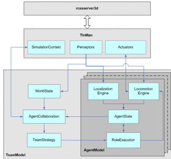
Fig. 1. Software Architecture
