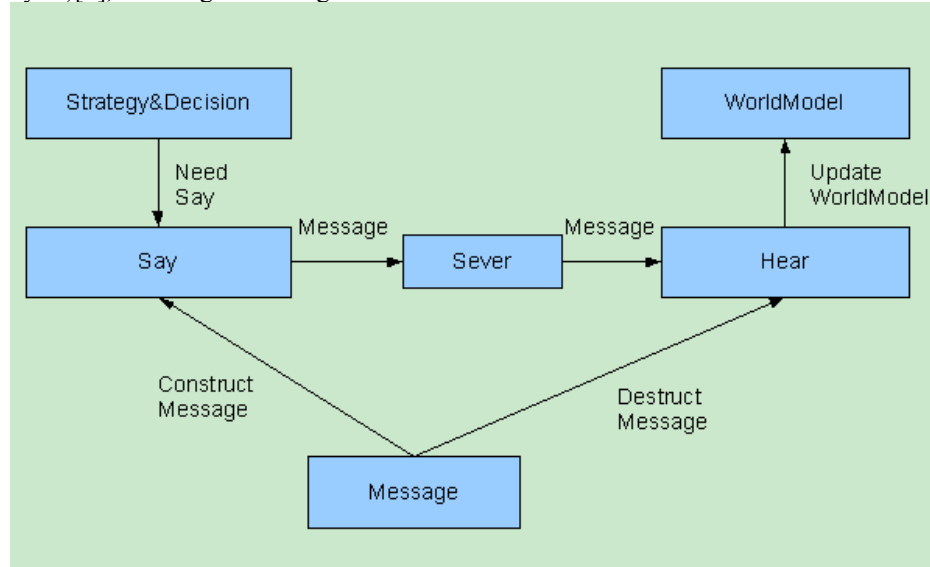
Fig.2. Communication Model
