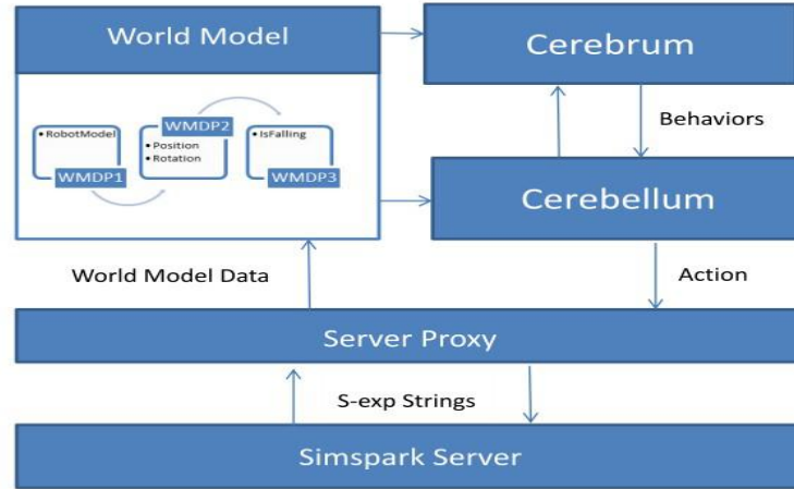
Fig. 1. Agent Architecture
