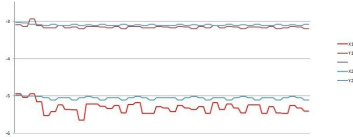
Fig. 3. Locating Results
