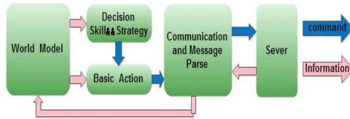
Fig. 1. AUA3D main running flow in about one cycle
