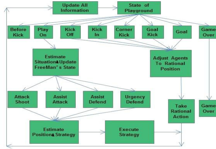
Fig. 2. Agent Strategy
