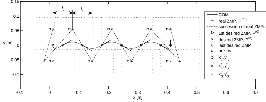
FIGURE 2. Forward walk of 0.4[m] from left to right. \ell_x is the step length. Footprints are in dotted lines. The COM trajectory is depicted. Successive real ZMPs are joined for better understanding.
