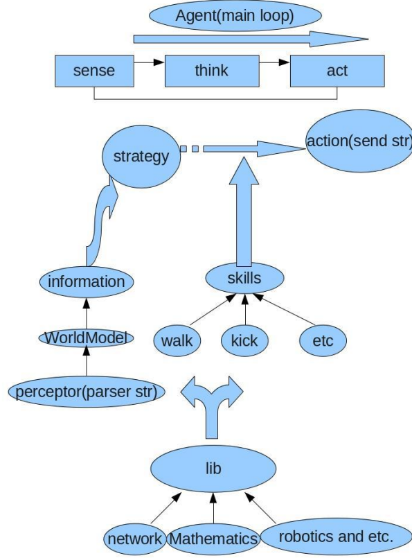
The main idea of our agent simulation
