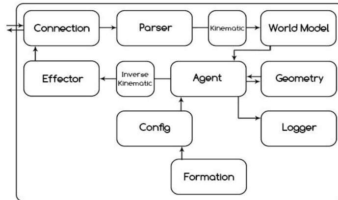
Fig. 1 . Scorpius Agent Architecture: Connection unit connects agent to the server, and passes data form server to the parser unit. Then WorldModel will be updated using these data. Also in order to obtain coordinates of each body section such as hands, legs and torso, it uses Kinematic unit. The agent makes a decision using WorldModel data, formation and geometry tools and sends it to the server by using some classes such as Effector and Connection.
