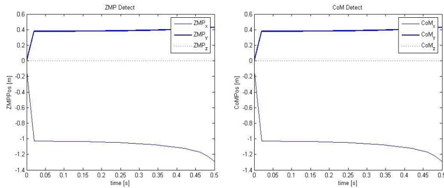
Fig. 6. Calculation of the ZMP and the COM
