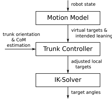
Fig. 1. Component diagram of a motion using the TcMF.
