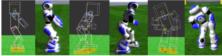
Fig. 2. Walk as an application of the TcMF. Image one and two: Nao upright. Image three and four: walking with 30 degrees forward leaning. Image five and six: walking with 20 degrees sideward leaning.
