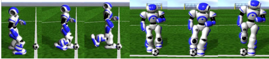
Fig. 3. Stop on one leg as an application of the TcMF. First image: end of final step motion. Second image: end of get on leg motion. Third image: end of balance on leg motion. Fourth to Sixth image: same from front.
