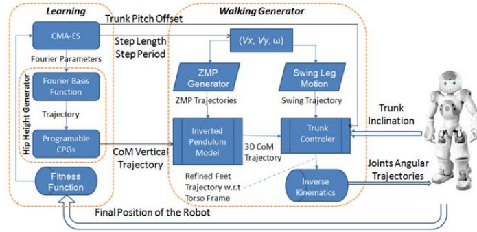
Fig 3. The interaction between each component of the proposed approach
