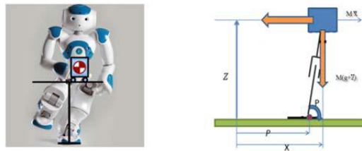
Fig. 1. Schematic view of inverted pendulum model on X direction and frontal view of the NAO robot
