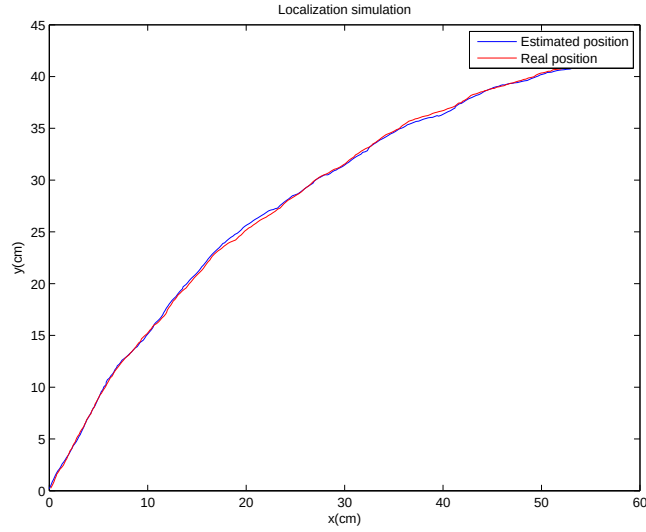
Fig. 3. Localization results.
